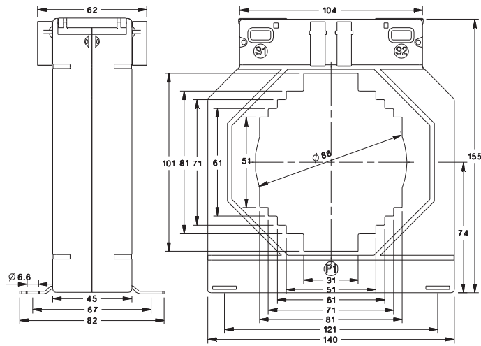
DIMENSIONAL DRAWING :
